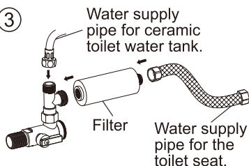
Water pipe valve connected to T valve.
